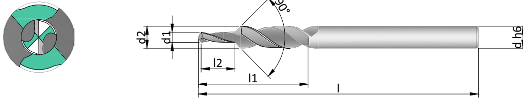
One step drill
