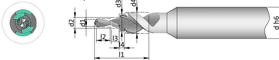
Three step drill
