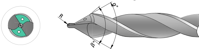
Form drill with radius and angles
